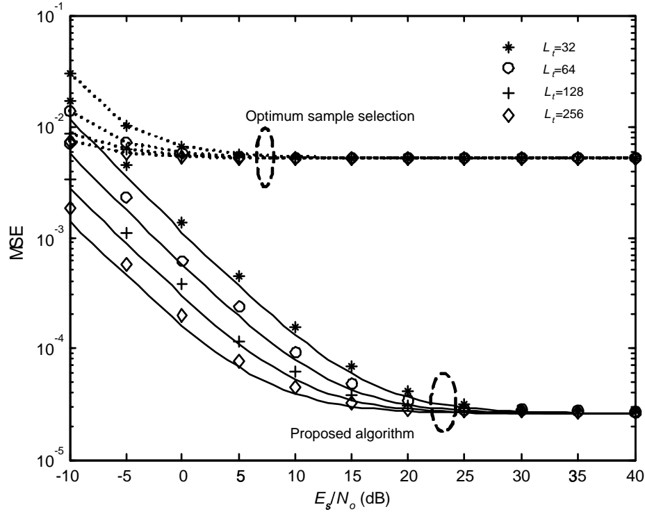
Fig. 5. MSE performance for different lengths of the training sequence ( N=2 , M=4 , Q=4 , \alpha=0.3 ).
