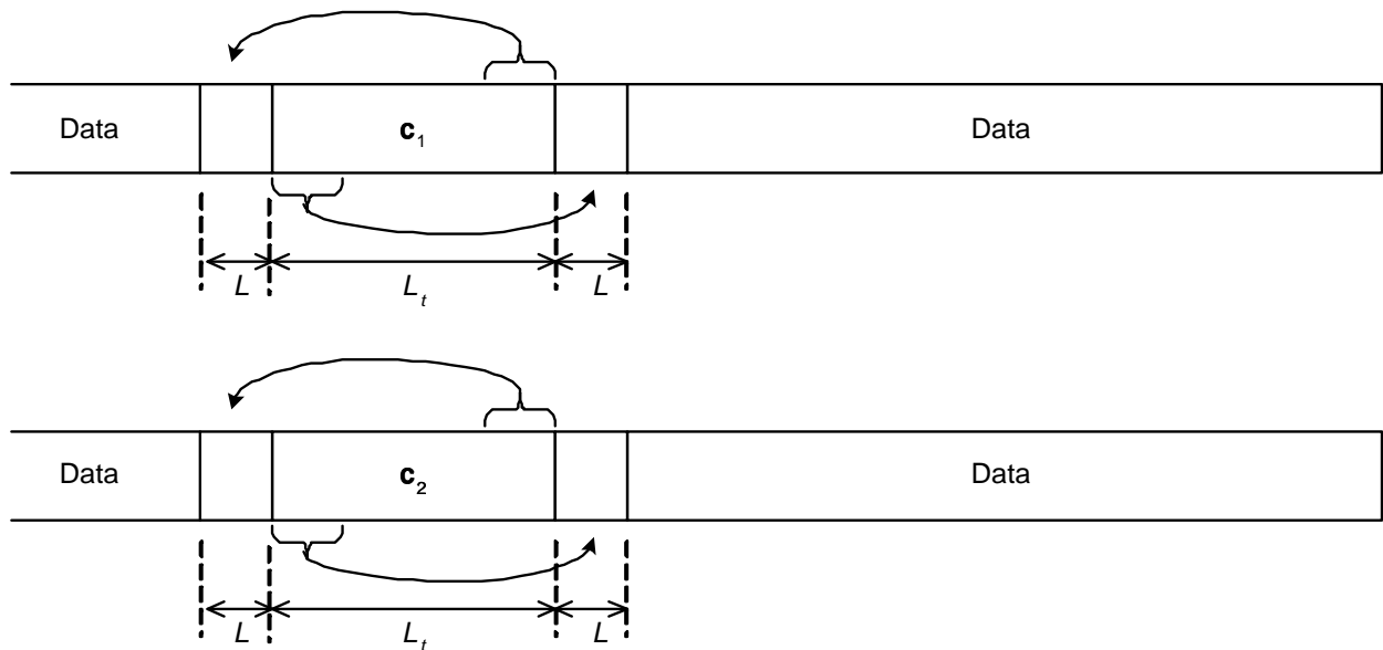
Fig. 2. Structure of the training sequence for symbol timing synchronization in a two transmit antennas system.
