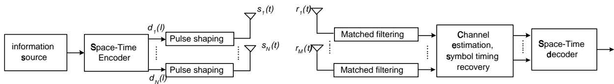
Fig. 1. Simplified baseband equivalent model for space-time coding system.
