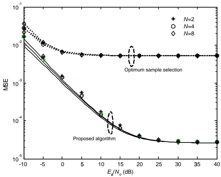
Fig. 7. MSE performance for different number of transmit antenna N ( L_t=64 , Q=4 , \alpha=0.3 , M=2 ).
