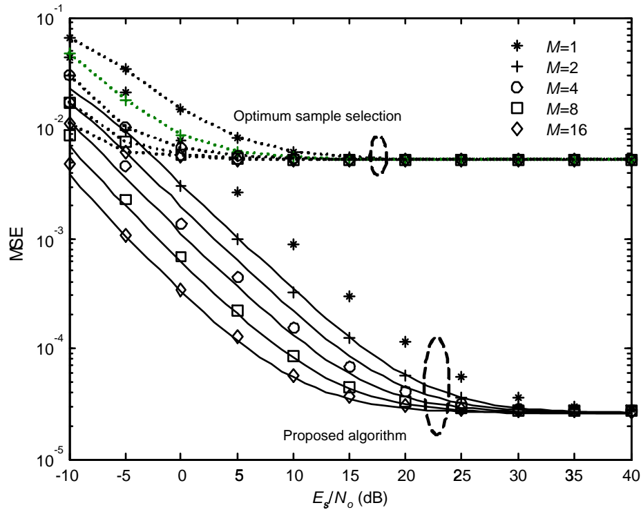
Fig. 6. MSE performance for different number of receive antenna M ( N=2 , L_t=32 , Q=4 , \alpha=0.3 ).
