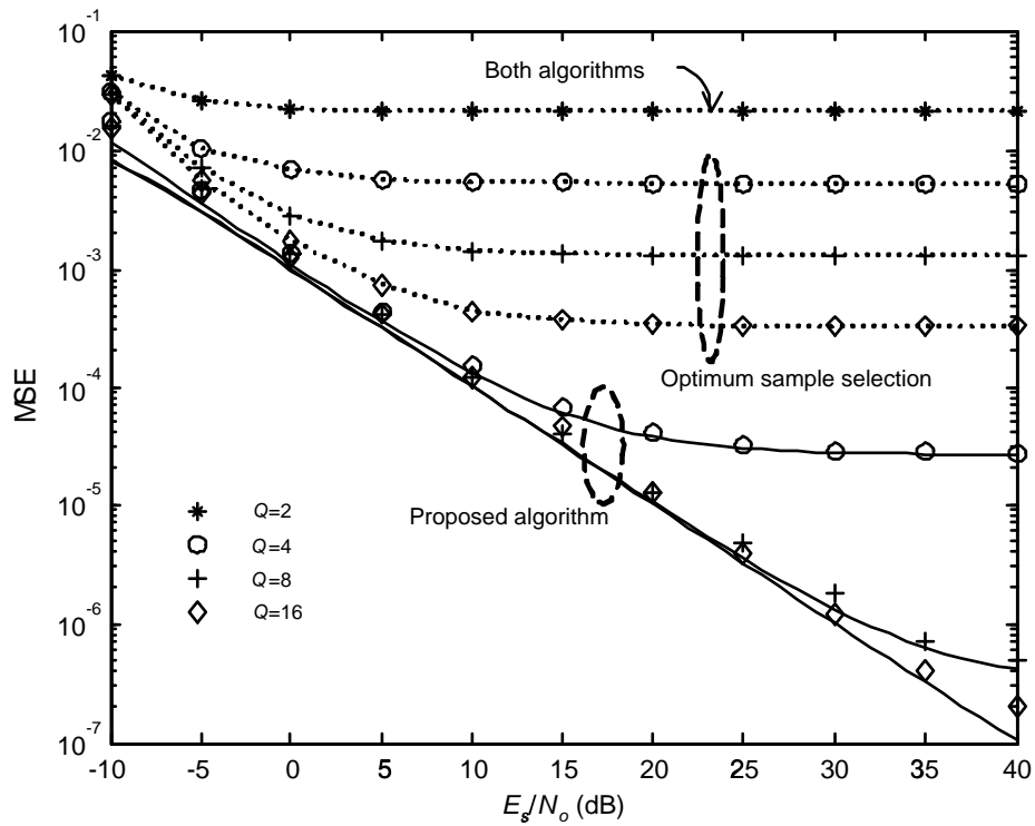
Fig. 4. MSE performance for different oversampling ratio Q ( N=2 , M=4 , L_t=32 , \alpha=0.3 ).
