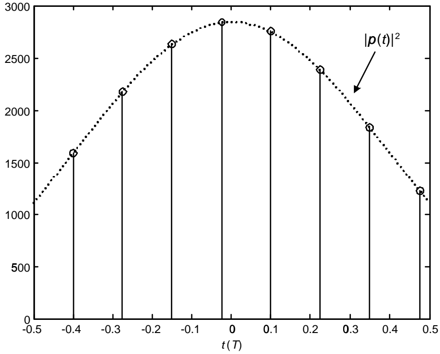
Fig. 3. An example of \Lambda_{ij}(k) with the scaled version of |p(t)|^2 for -T/2 \leq t \leq T/2 (dotted line).
